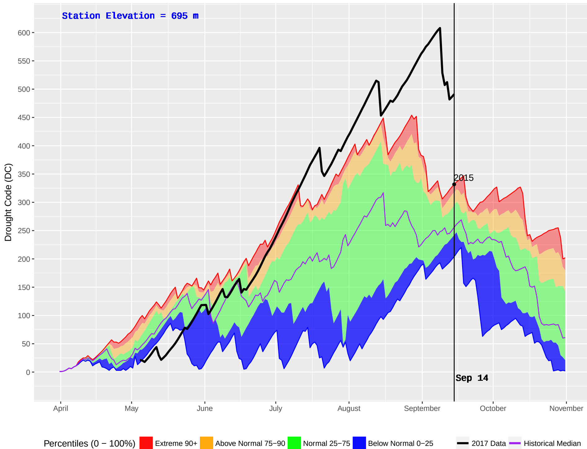
BLUE RIVER 2 (1108) : Historical (2011–2016) and Current (2017) Noon Drought Code (DC)
