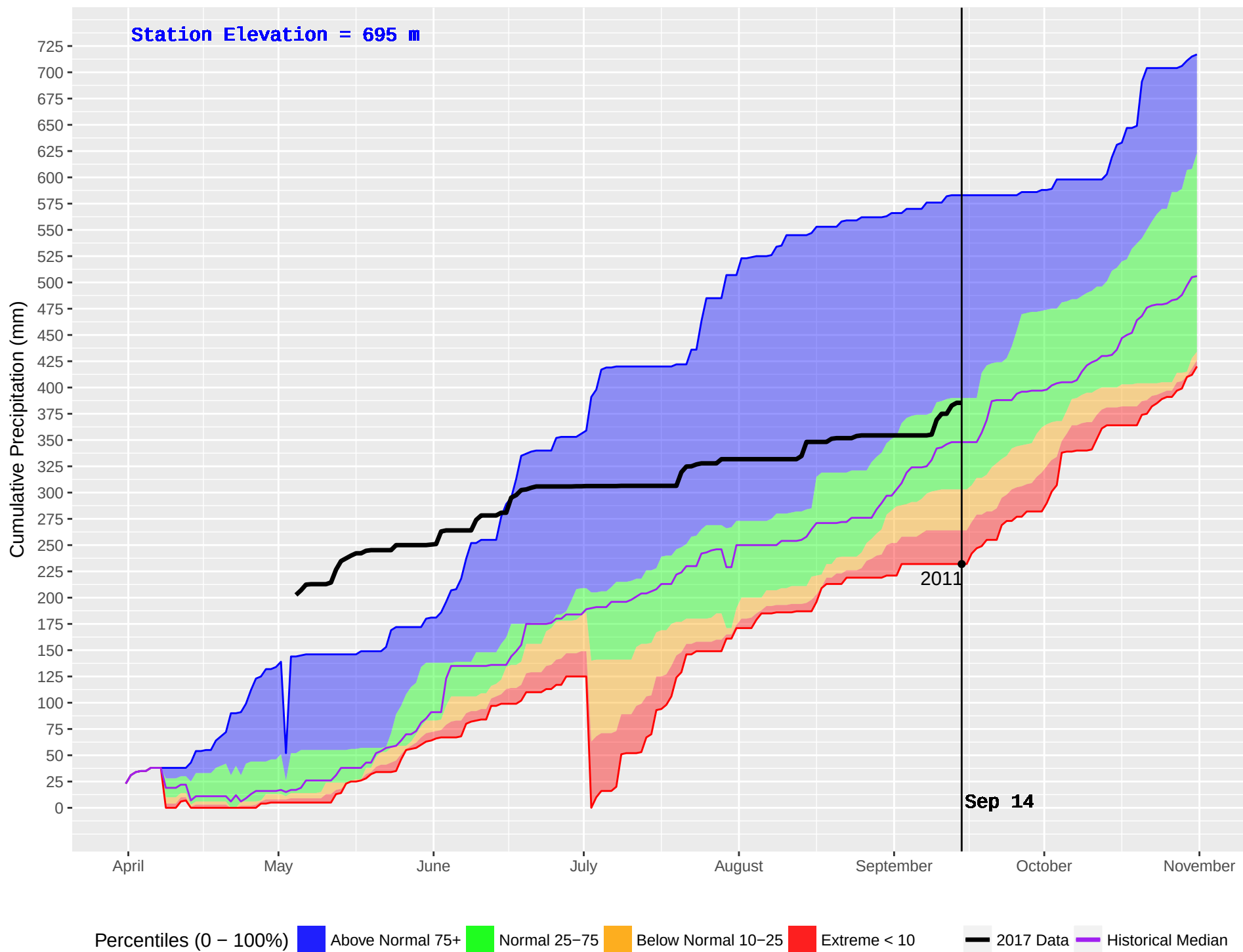
BLUE RIVER 2 (1108) : Historical (2011–2016) and Current (2017) Noon Cumulative Precipitation
