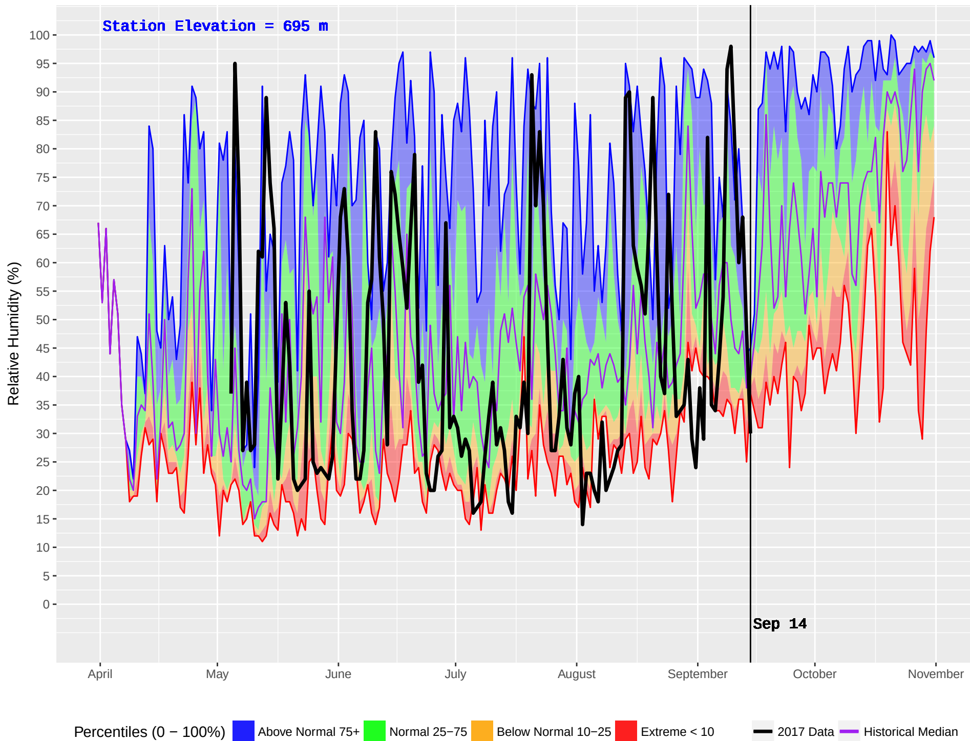
BLUE RIVER 2 (1108) : Historical (2011–2016) and Current (2017) Noon Relative Humidity
