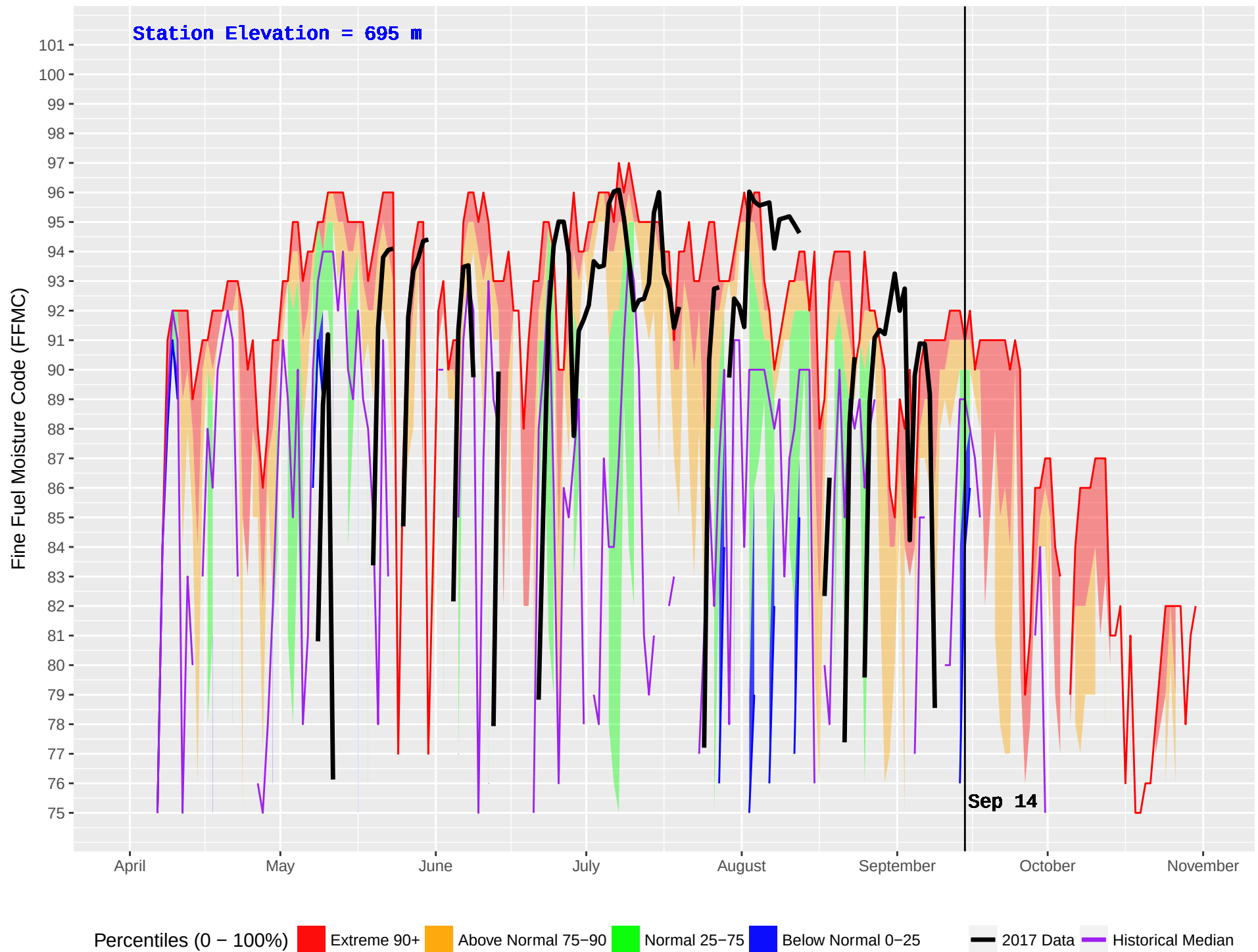
BLUE RIVER 2 (1108) : Historical (2011–2016) and Current (2017) Noon Fine Fuel Moisture Code (FFMC)
